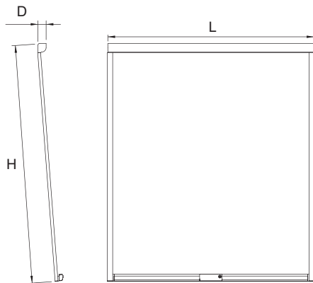
SC-DX Plan View
