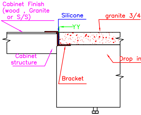
TOP BRACKET DETAIL
