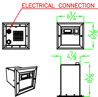
PANEL CONTROL
