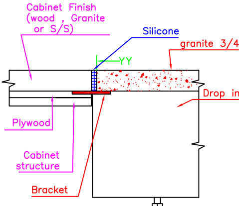
BOTTOM BRACKET DETAIL Flush
